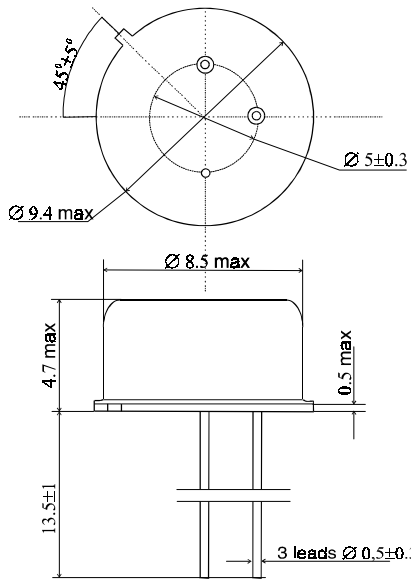
TO 39
