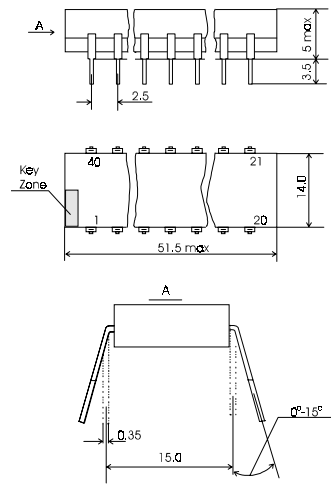
2123.40-2(40-pin Plastic DIP)
